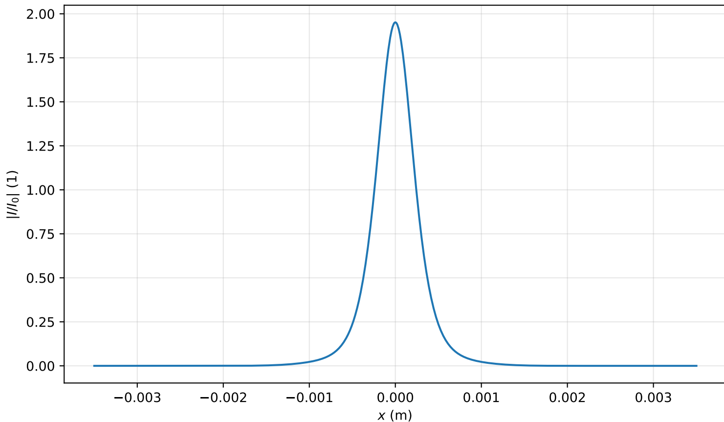
Intensity profile I(x, y = 0, z = 1.672m)/I_0 , P_{in}=1.0P_{cr} , artificial time
